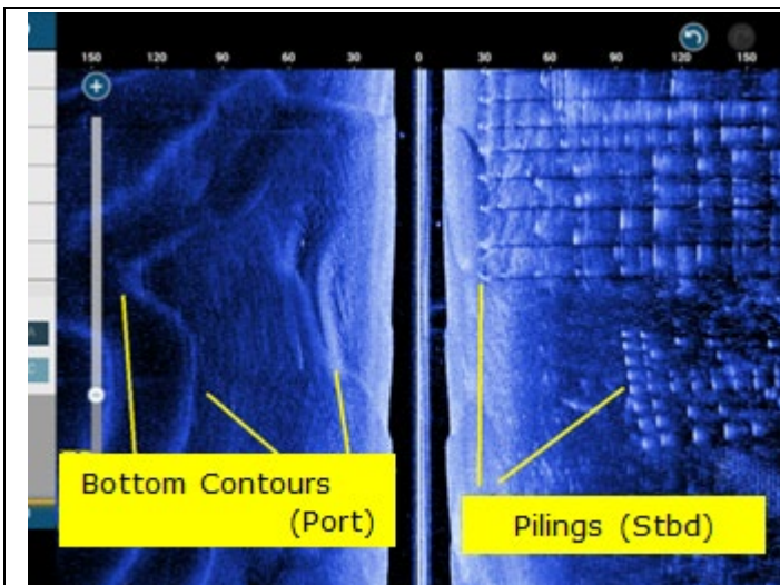
While pillings at the harbor is observed at starboard, you can also see the shape and contour of bottom at port.
