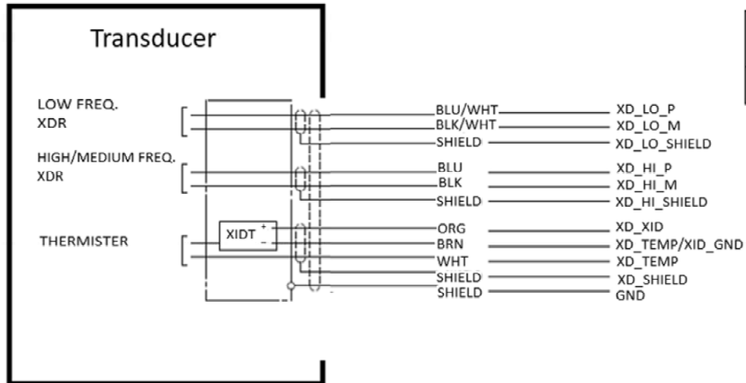
Model of transducers associated with wiring diagram
