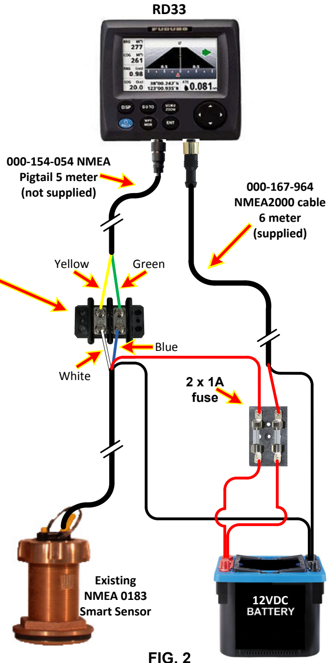
NEW RD33 DISPLAY WITH NMEA 0183 SMART SENSOR
