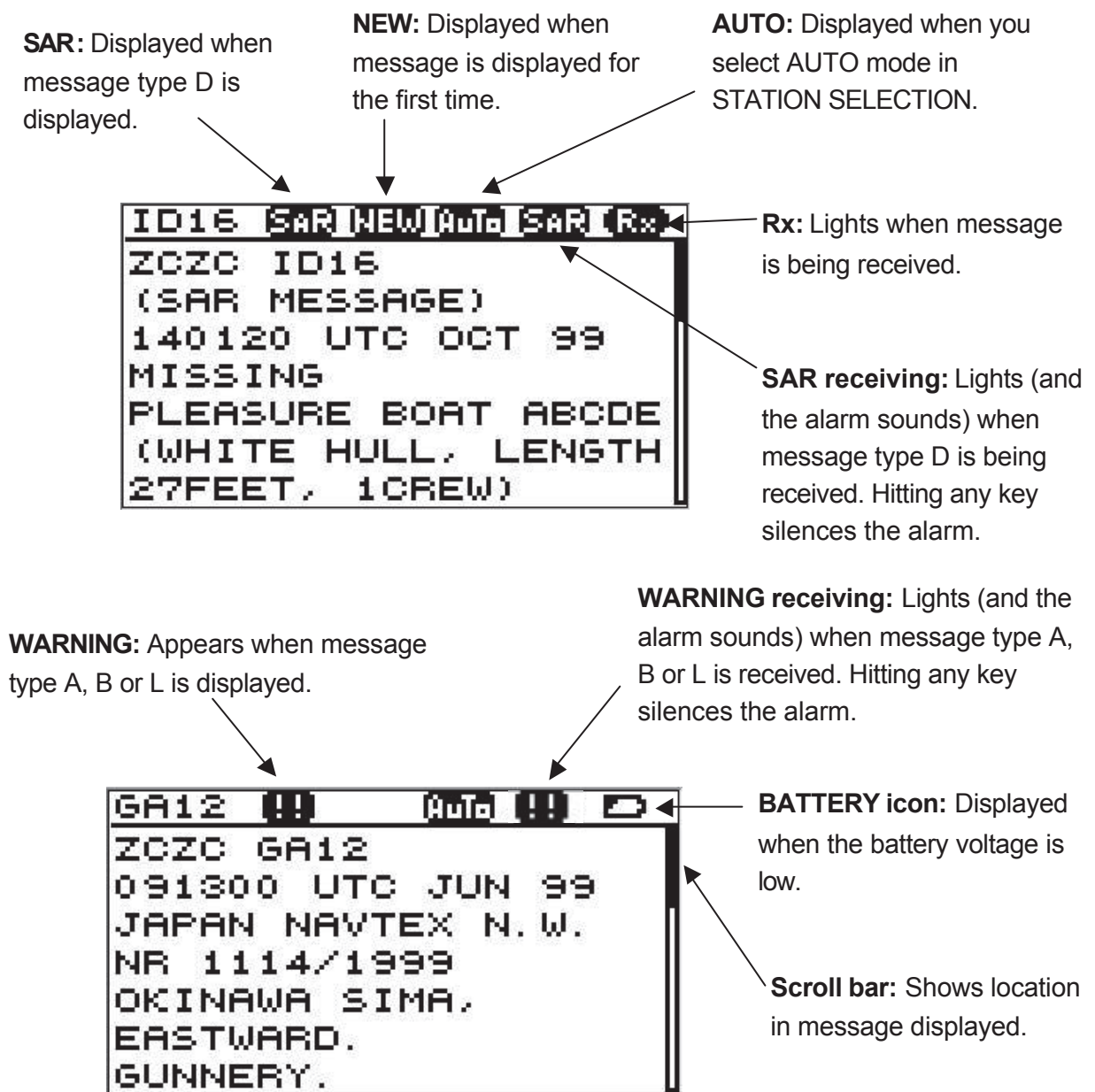
Figure 1-2 Display indications
