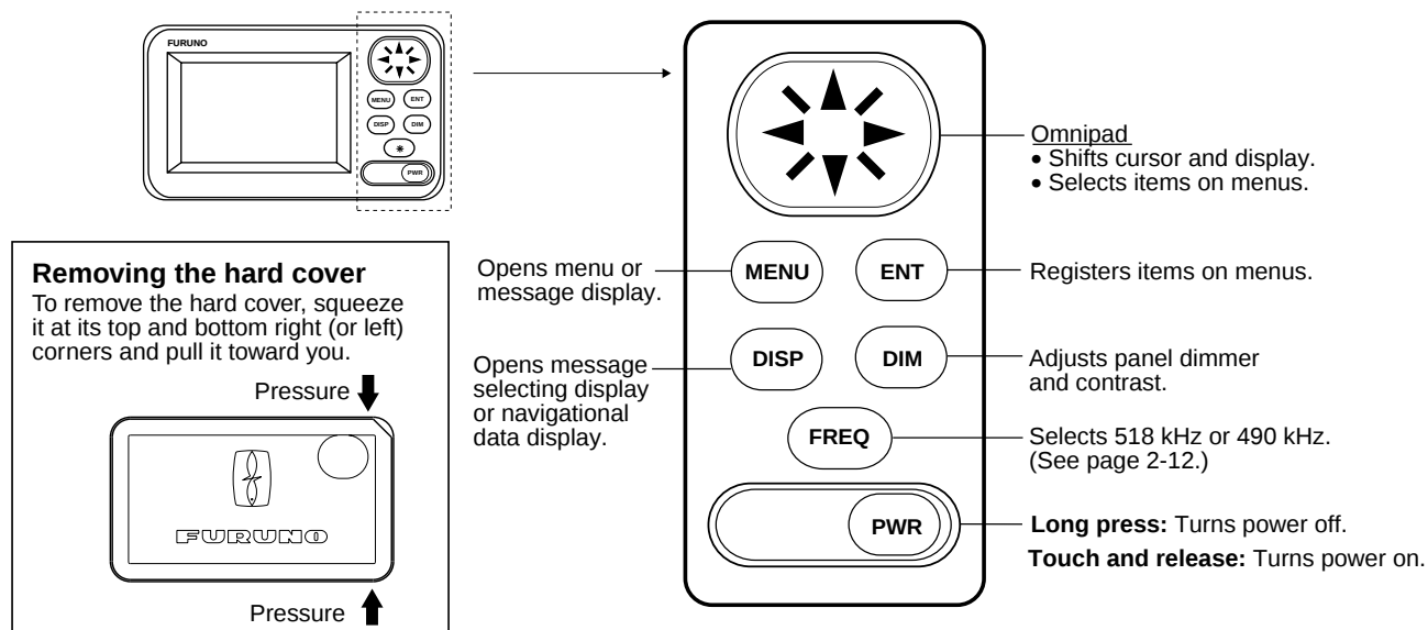
Figure 2-1 Control panel
