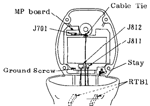
Fig.9 Internal Wirings
