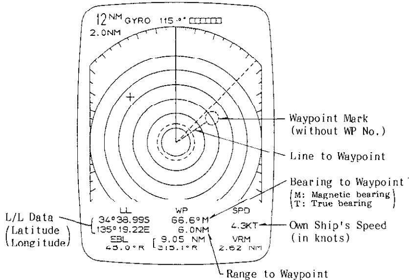
Fig.35 Nav Data on the Screen
