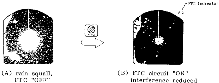
Fig.29 Precipitation Interference
