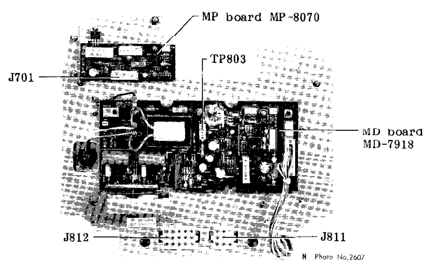
Fig.54 Transceiver Module Bottom view (Shield cover removed)
