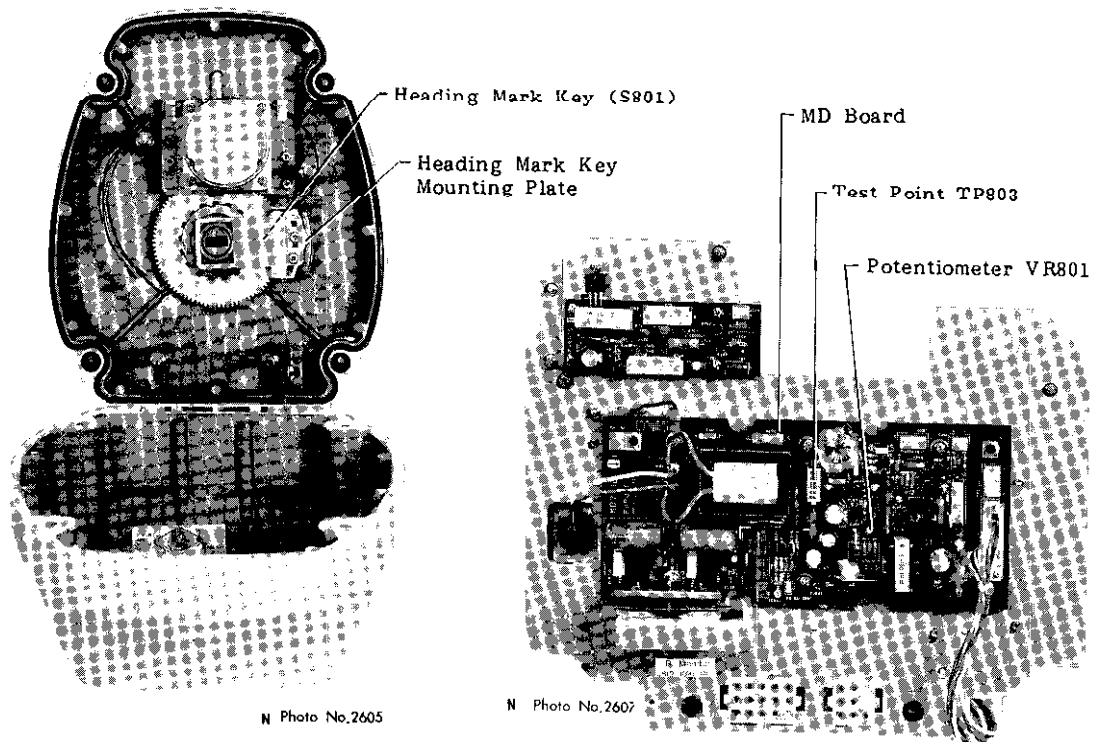
(a) Transceiver module removed
