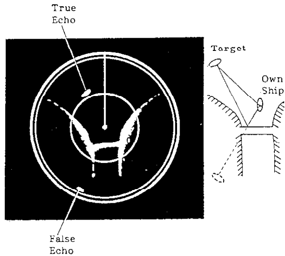
Fig.43 Indirect Echoes
