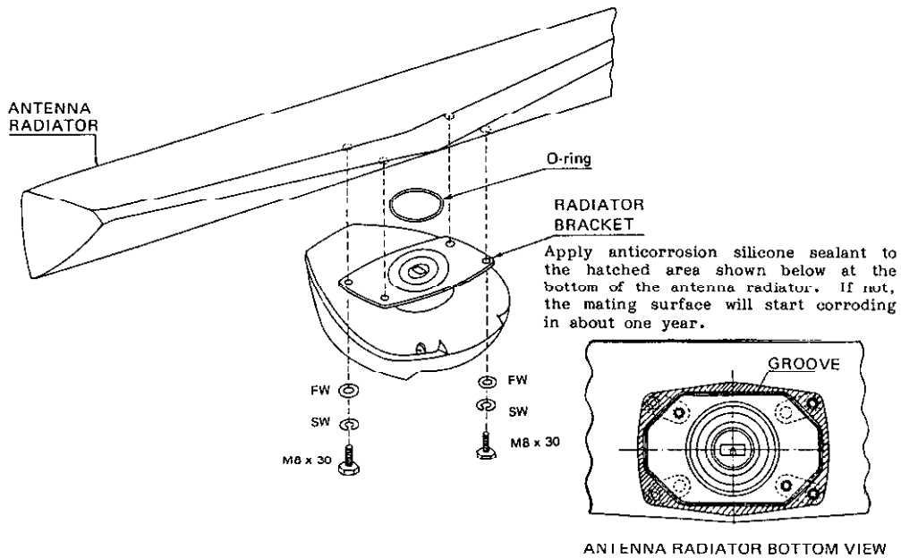
Fig.8 Antenna Radiator Mounting
