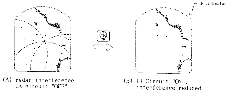
Fig.30 Radar Interference
