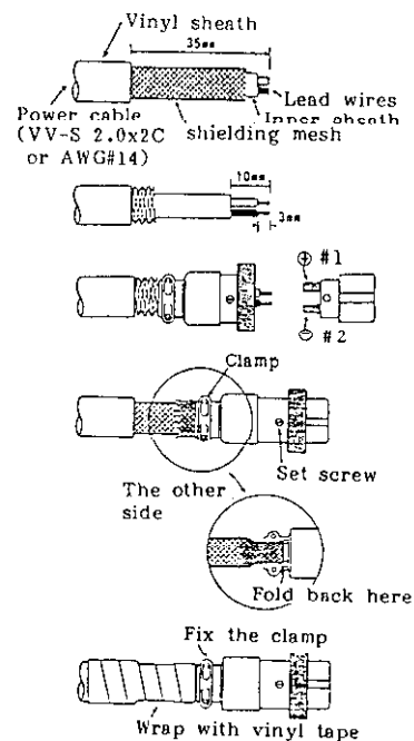
Fig.11 Power Connector Assy.
