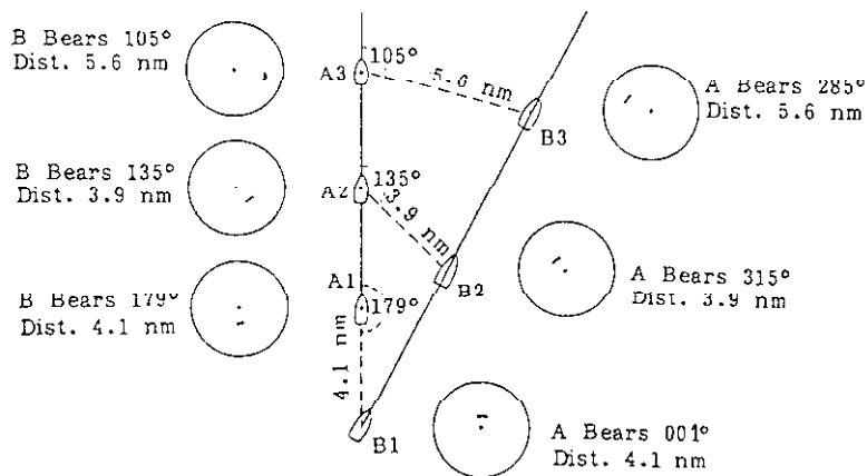
Fig.48 Relative Motion vs. True Motion
