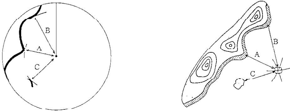
Fig.45 Position Fixing Using Radar Ranges
