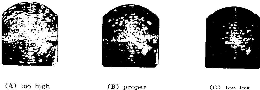
Fig.24 Setting the Gain Control
