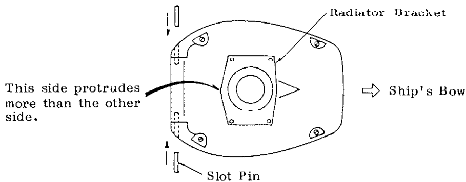
Fig.7 Slot Pin Insertion
