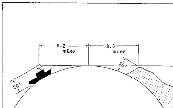
Fig.38 Radar Horizon
