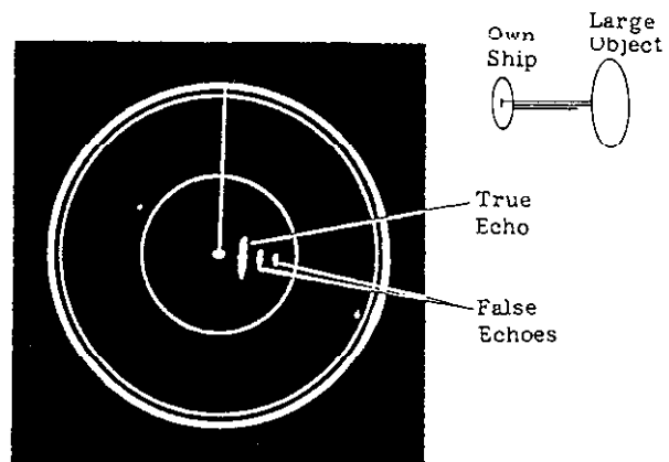
Fig.40 Multiple Echoes
