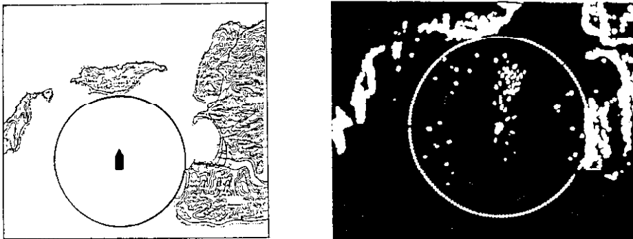
Fig.44 Navigation Chart and Corresponding Radar Picture
