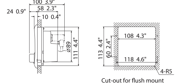
NAVpilot-711 Control Unit (Flush-mount) 0.35 kg 0.77 lb
