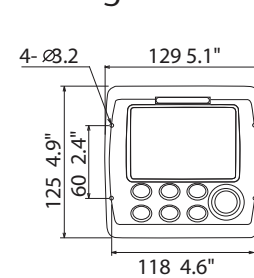
NAVpilot-711 Control Unit (Flush-mount) 0.35 kg 0.77 lb
