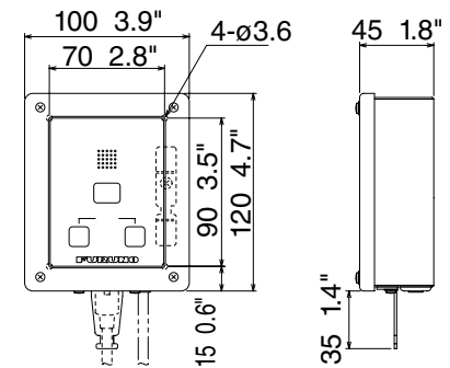
FELCOM250/500 Incoming Indicator FB-3000
