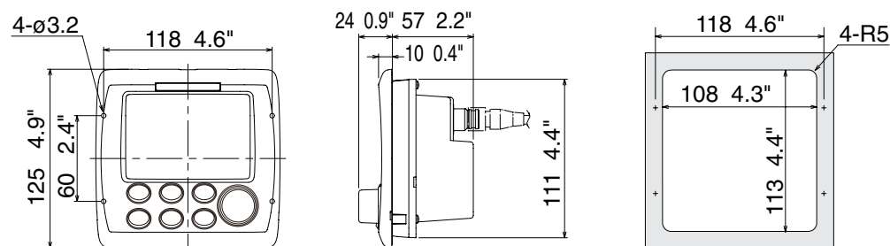
NAVpilot 511 Optional Control Unit (Flush Mount)
